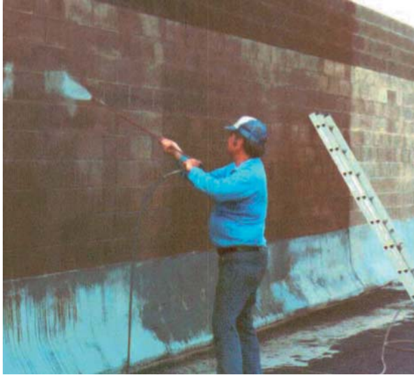
Surface Shield being applied to a concrete block sound barrier
